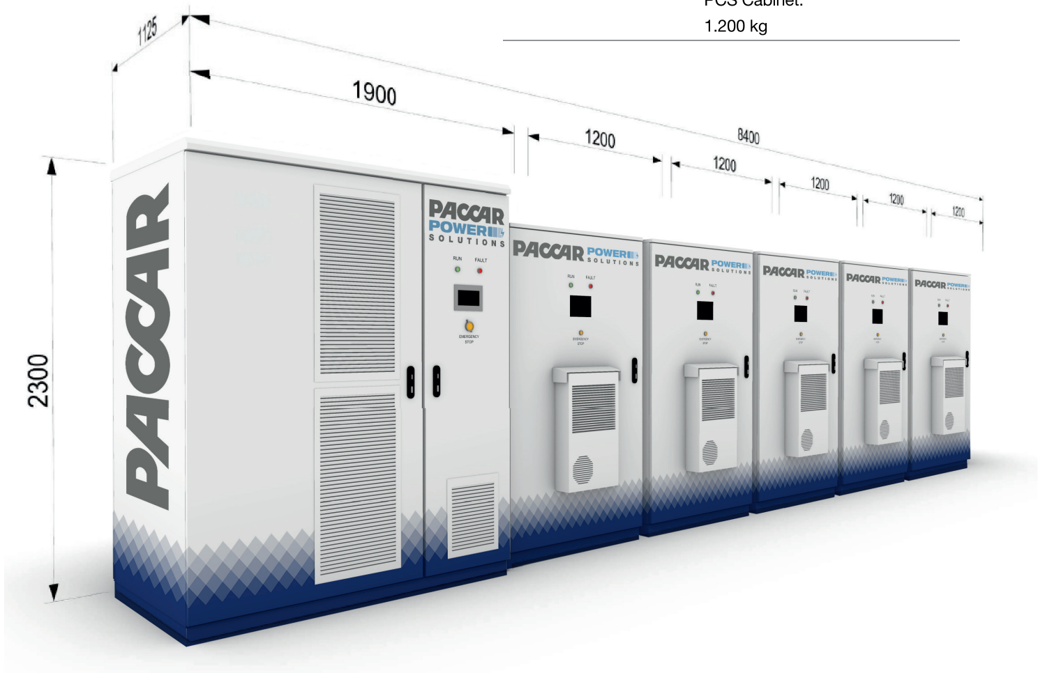
System example: 1 PCS + 5 Battery cabinets configuration
